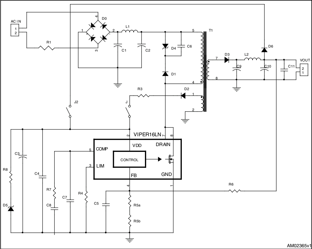
Figure 1. Application schematic
